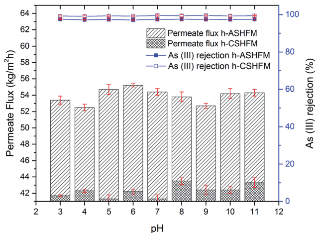
Fig. 4 Effect of pH on the permeate flux and As(III) rejection of h-ASHFM and h-CSHFm sintered at 1200^\circ\text{C} , during the DCMD process (number of samples, n = 3 ; arsenic concentration = 1 ppm; arsenic feed temperature = 60^\circ\text{C} ).
