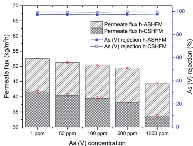
Fig. 7 Effect of As(V) concentration on the permeate flux and As(V) rejection of h-ASHFM and h-CSHFm sintered at 1200 °C, during the DCMMD process (number of samples, n = 3 ; arsenic feed temperature = 60 °C; arsenic pH = 7.45).
