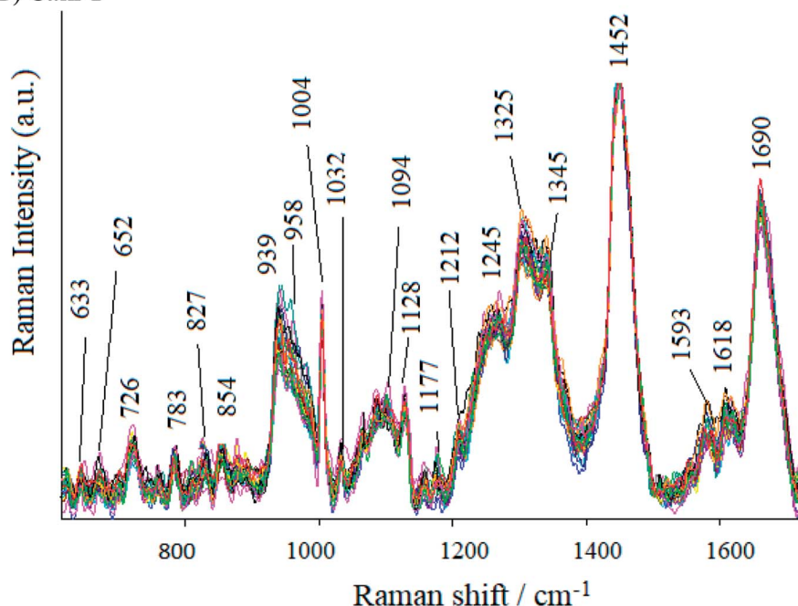
Fig. 7 (A) The SERS spectra of B. subtilis and (B) Caki-1 recorded on Ag/PV substrate in mapping mode from 40 different points in mapping mode ( 10 \times 20 \mu\text{m} ). For all spectra, excitation wavelength was at 785 nm, laser power was 1.5 mW, and acquisition time was only 3 seconds.
