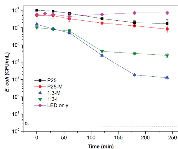
Fig. 6 Bacterial disinfection with P25, P25-M and FeOOH-TiO 2 1 : 3 composites under visible light at 300 mg L -1 .
