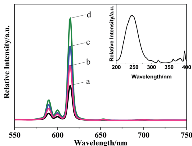
Fig. 6 The emission spectra of \text{Ba}_3[\text{Ge}_2\text{B}_7\text{O}_{16}(\text{OH})_2](\text{OH})(\text{H}_2\text{O})\text{:Eu}^{3+} prepared for different reaction times ( \lambda_{\text{ex}} = 242\text{ nm} ): (a) 24\text{ h} , (b) 48\text{ h} , (c) 72\text{ h} , and (d) 96\text{ h} .
