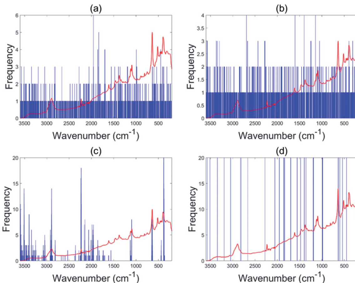
Fig. 7 Variables selected by the different methods for the Raman tablet data: BSS (a), GA-PLS-DA (b), s-PLS-DA (c) and EBSS (d).
