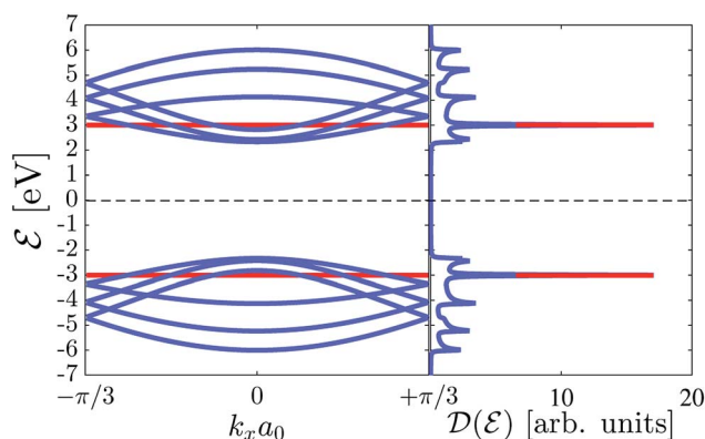
Fig. 2 The electronic band structure (left panel) and density of states (right panel) of the 7-aBNNR. The band gap is about 4.5 eV. In the electronic DOS panel, the van Hove singularities corresponding to the flat bands are shown by the red peaks, i.e. the degenerate states. The dashed line is the Fermi level.
