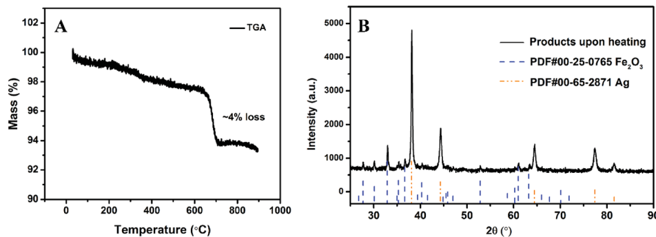
Fig. 2 (A) TGA of \text{AgFeO}_2 in Ar at a heating rate of 10\text{ °C min}^{-1} ; (B) \text{AgFeO}_2 decomposition product after heating to 1000\text{ °C} .
