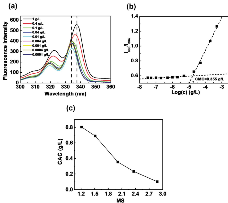
Fig. 2 (a) Excitation spectra of pyrene ( 6 \times 10^{-7} mol \text{L}^{-1} ) in water in the presence of increasing concentrations of HIPEC-3 ( \lambda_{\text{em}} = 490 nm). Measurements were performed at 10 °C. (b) Plot of I_{338}/I_{334} in the excitation spectra versus the concentration of HIPEC-3. (c) Effect of MS on CAC.
