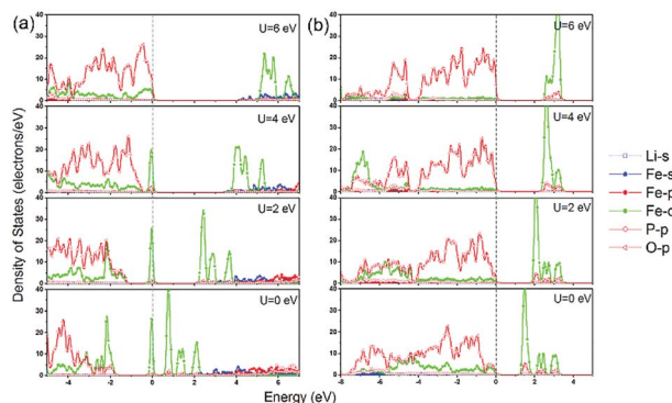
Fig. 7 Partial density of states (PDOS) calculated in GGA and GGA+ U for (a) LiFePO 4 and (b) FePO 4 with AFM configuration.
