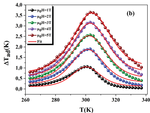
Fig. 10 \Delta T_{\text{ad}} plotted as a function of temperature at different \mu_0 H fields, for x = 0.15 and 0.20 compounds. The red line curves represent the modeled data and symbols are the experimental data.
