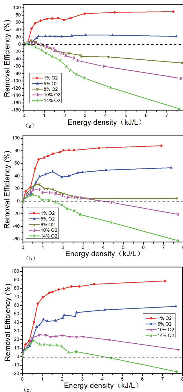
Fig. 12 Denitration performance of NTP in NO/NH_3/O_2/N_2 system, (a) 500 \mu L L^{-1} NO + 500 \mu L L^{-1} NH_3 + O_2 , (b) 1000 \mu L L^{-1} NO + 1000 \mu L L^{-1} NH_3 + O_2 , (c) 1500 \mu L L^{-1} NO + 1500 \mu L L^{-1} NH_3 + O_2 .
