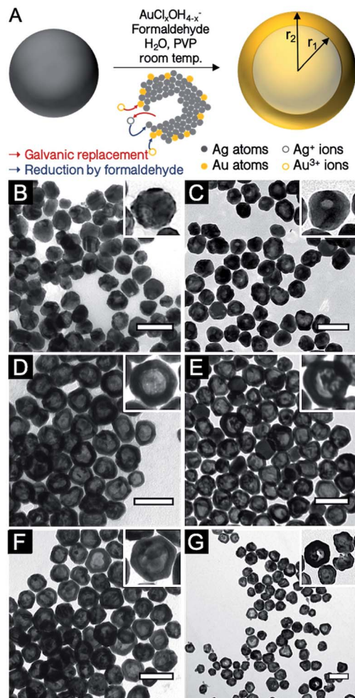
Fig. 1 (A) Schematic illustration of the co-reduction galvanic replacement procedure used. (B–G) TEM images of reaction products for different Au:Ag stoichiometries (B) 0.1Au:Ag, (C) 0.25Au:Ag, (D) 0.50Au:Ag, (E) 0.75Au:Ag, (F) Au:Ag, and (G) 2Au:Ag. Scale bars, 100 nm.
