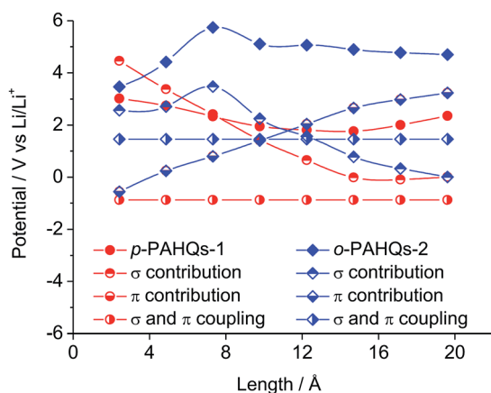
Fig. 5 The contributions of \sigma bond, \pi bond, \sigma and \pi coupling coefficient to the redox potential of p -PAHQs-1 and o -PAHQs-2.
