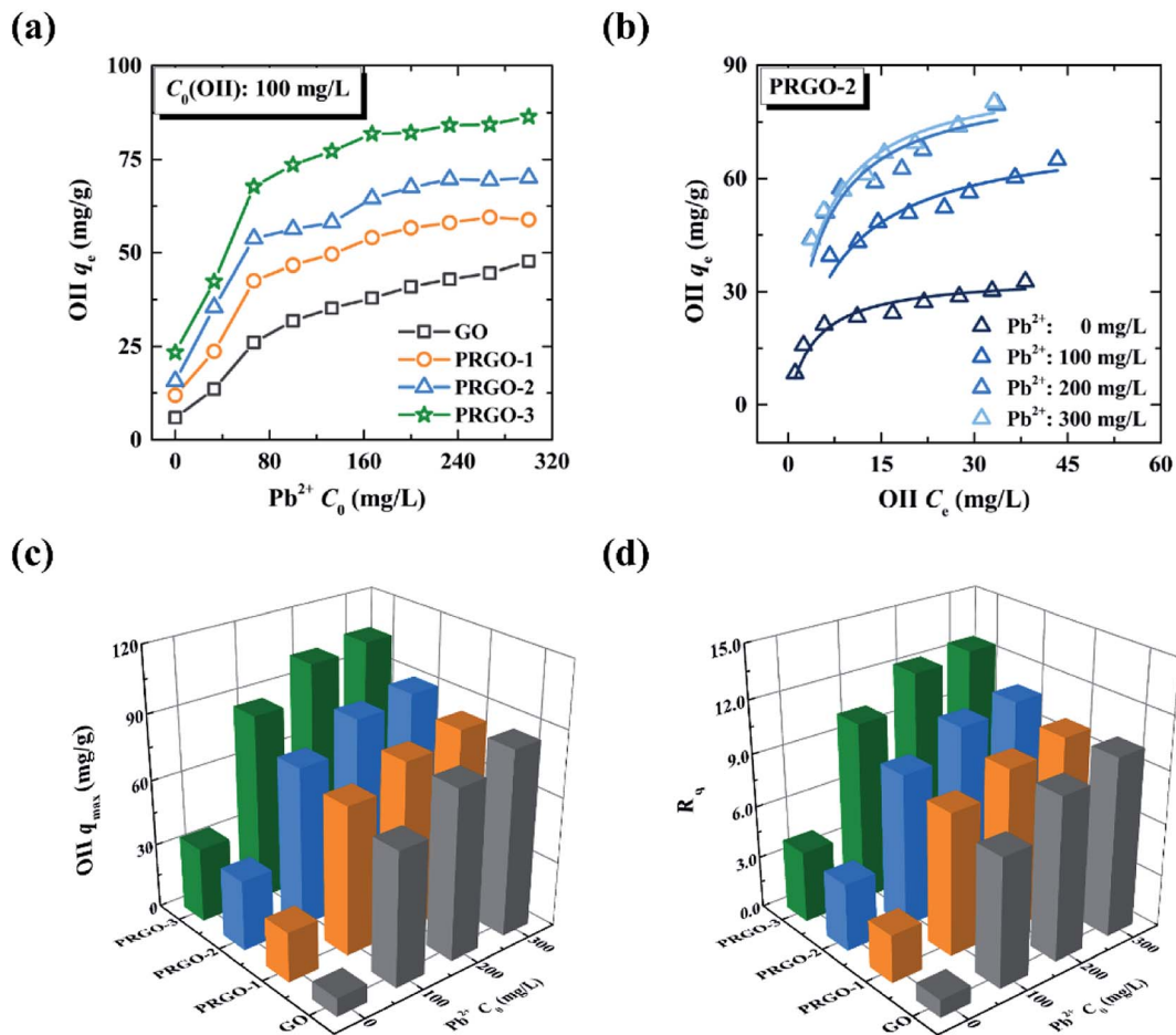
Fig. 7 Co-adsorption of OII in the presence of Pb^{2+} . (a) The equilibrium adsorption capacities of OII on GO and PRGO as a function of Pb^{2+} concentration. (b) The adsorption isotherms of OII on PRGO-2 under different Pb^{2+} concentrations. The solid lines are the Langmuir model simulations. (c) The maximum adsorption capacities of OII on GO and PRGO in the presence of Pb^{2+} . (d) The corresponding ratios R_q of OII on GO and PRGO in the presence of Pb^{2+} .
