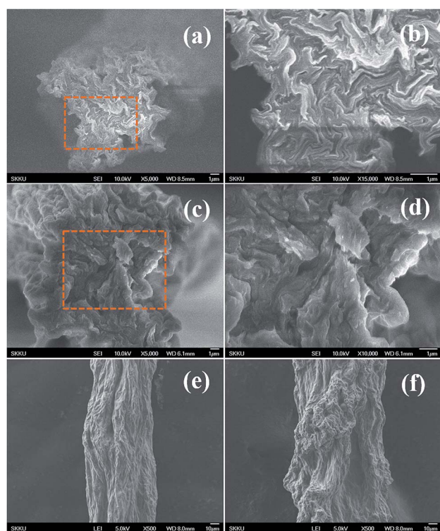
Fig. 3 SEM images of EGO and GO fibers. Cross-sections of (a) EGO, (c) GO fibers, surface morphologies of (e) EGO and (f) GO fibers.
