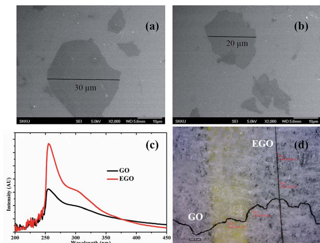
Fig. 2 SEM images of (a) EGO and (b) GO sheets. (c) UV-visible of GO and EGO. (d) Optical image of EGO and GO fibers.
