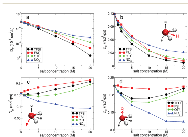
Fig. 10 Translational and rotational diffusion constants of water molecules. (a) Translational diffusion constant D_T of water molecules as a function of salt concentration for different anions in a semi-log plot. For subdiffusive translations, we estimate D_T by simply calculating the slope of TMSD (divided by 6) in Fig. 9. (b) Rotational diffusion constant D_{R,H} of a polarization vector \vec{H} of a water molecule as a function of salt concentration for different anions. (c) Rotational diffusion constant D_{R,P} of a principal vector \vec{P} of a water molecule as a function of salt concentration. (d) Rotational diffusion constant D_{R,Q} of a principal vector \vec{Q} of a water molecule as a function of salt concentration.
