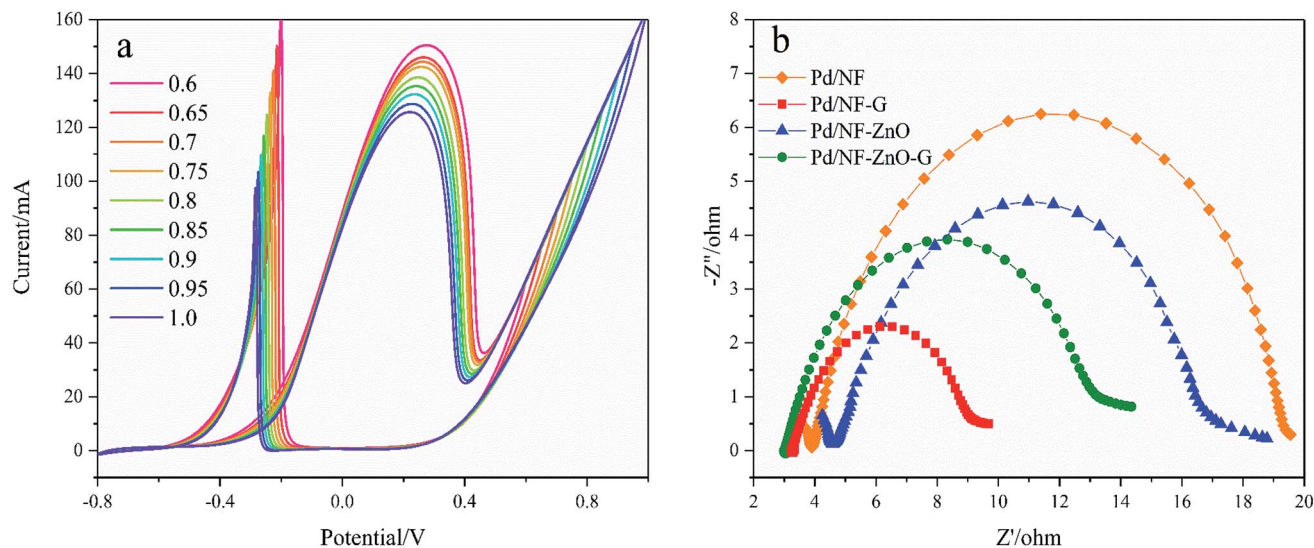
Fig. 8 (a) CVs of Pd/NF-ZnO-G in 1 M KOH containing 0.5 M glucose for different upper scanning limits at a scanning rate of 50 \text{ mV s}^{-1} ; (b) Nyquist plots of Pd/NF, Pd/NF-G, Pd/NF-ZnO and Pd/NF-ZnO-G in 0.1 M KOH + 0.1 M glucose at 0.3 V in the frequency range between 0.05 Hz and 10^5 Hz.
