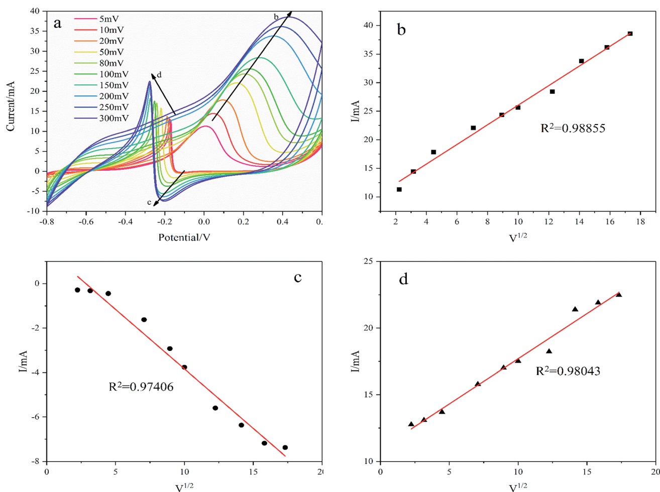
Fig. 9 (a) CVs of Pd/NF-ZnO-G at scanning rates of 5, 10, 20, 50, 80, 100, 150, 200, 250, and 300 \text{ mV s}^{-1} in 0.1 M KOH containing 0.5 M glucose; (b), (c) and (d) calibration plots showing the linear relationship between the square root of the potential scan rate ( v^{1/2} ) vs. peak current ( I ).
