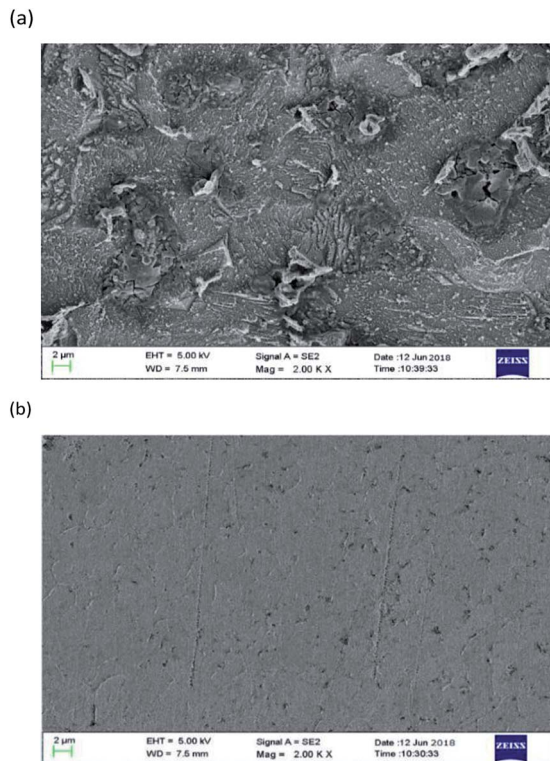
Fig. 11 SEM images of mild steel surfaces: (a) 1 M HCl and (b) PTA.
