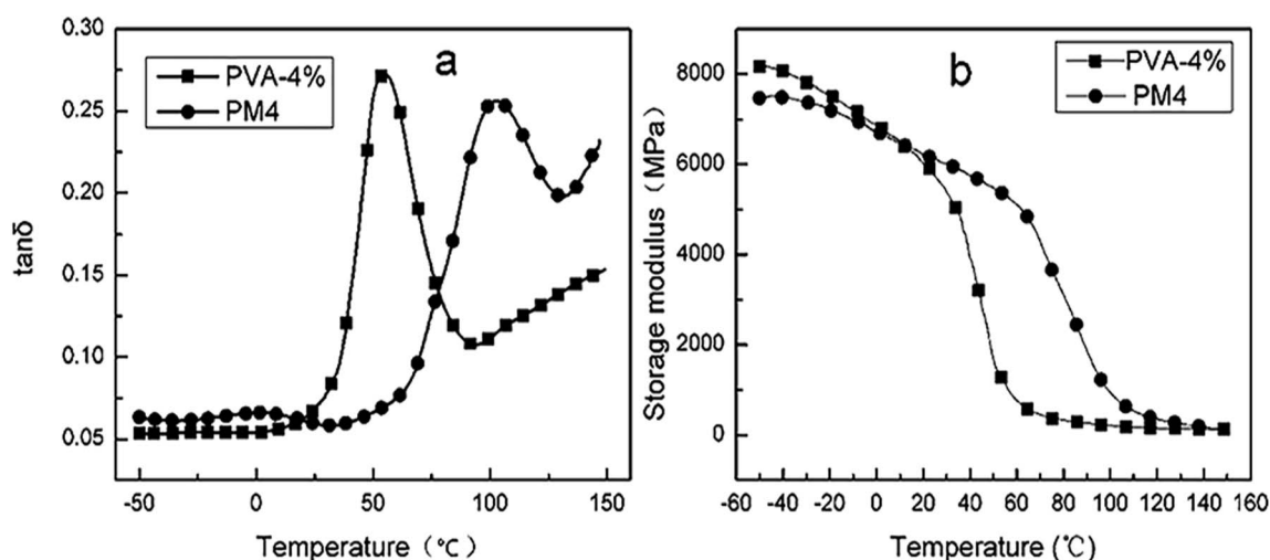
Fig. 12 Plots of \tan \delta and storage modulus G' against temperature of PVA with 4% content of water and MgCl_2 \cdot 6H_2O , respectively.
