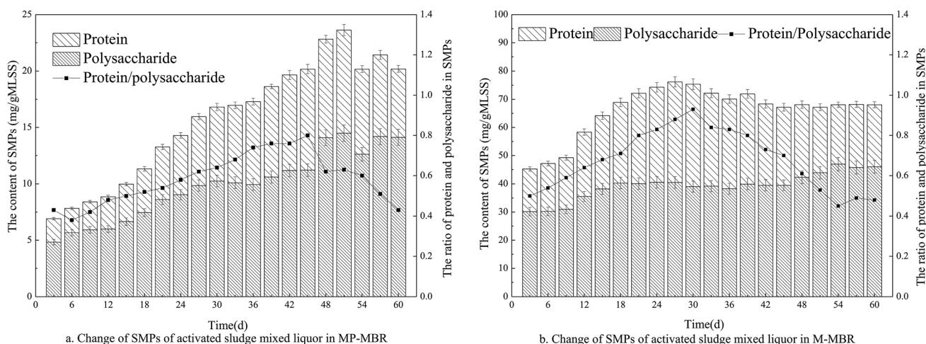
Fig. 4 Change in the content of SMPs of activated sludge mixed liquor.
