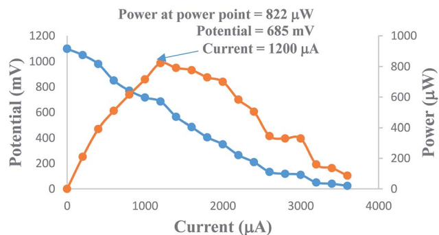
Fig. 2 Variation of the potential and power with the i - V characteristics of the cell. (1) Potential vs. current (nearly linear curve). (2) Power vs. current (inverted, nearly V-shaped curve).
