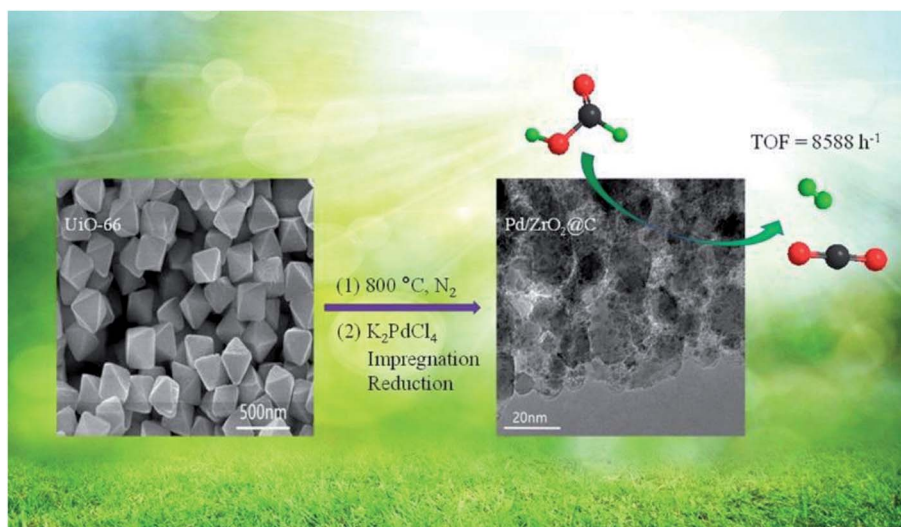
Scheme 1 Schematic illustration for the preparation of \text{Pd/ZrO}_2\text{@C} .
