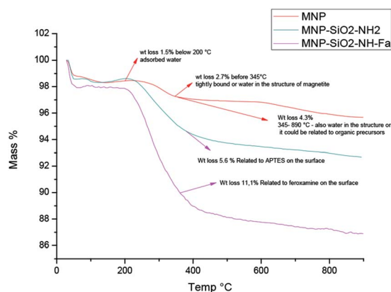
Fig. 5 Thermogravimetric analysis of MNP (red), \text{MNP@SiO}_2@\text{NH}_2 (green), and \text{MNP@SiO}_2@\text{NH@Fa} (4) (pink).
