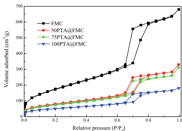
Fig. 1 \text{N}_2 adsorption/desorption isotherms of the PTA@FMC materials.
