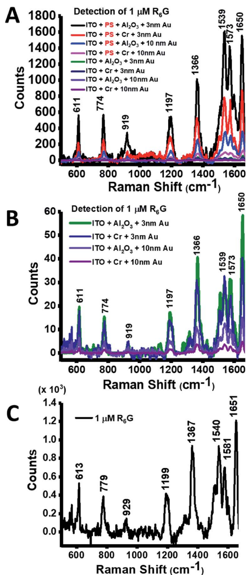
Fig. 5 (A) SERS spectra of the Au/ITO compared to Au deposition on ITO without a PS template, (B) the zoomed image of Au deposition on ITO without a PS template, (C) normal Raman spectrum of 1 μM R 6 G.
