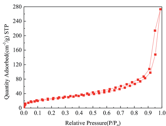
Fig. 7 N 2 adsorption and desorption isotherm of Fe 3 O 4 @SiO 2 -g-PAMAM-AO.
