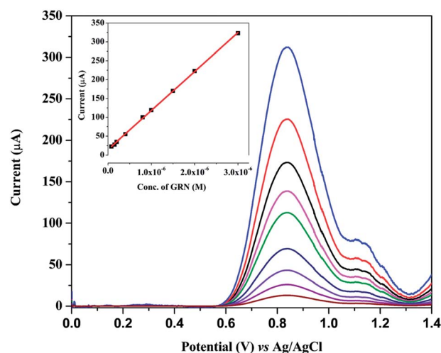
Fig. 10 Square wave voltammograms for different concentrations of GRN (0.08 to 3.0 μM). Optimum parameters: 0.04 M BR buffer (pH = 7.0), E_{acc} = -0.2 V, frequency = 250 Hz, pulse height = 10 mV, step height = 10 mV and t_{acc} = 120 s. Inset: calibration curve between concentration and peak current.
