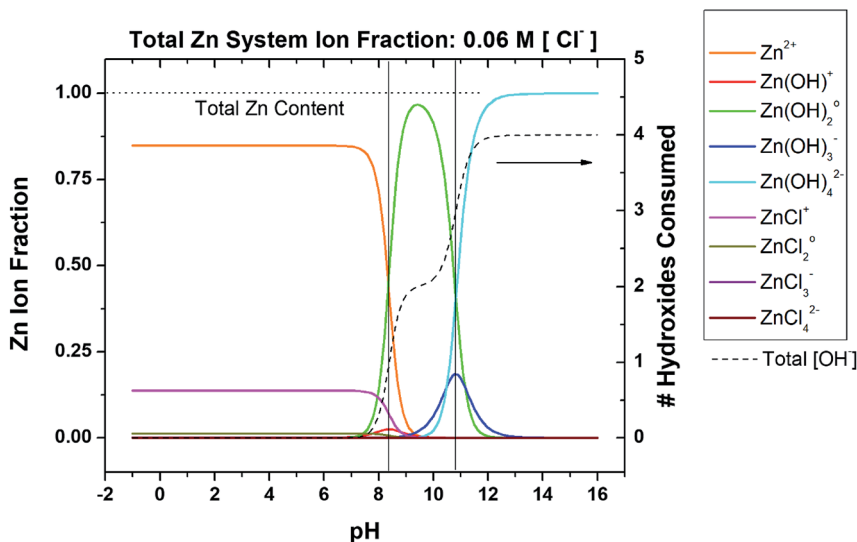
Fig. 2 Speciation diagram depicting the fractional distribution of various Zn-based species as a function of pH for a given ligand concentration, in this case 0.06 M [Cl - ]. Included is the function (dashed line) which describes the number of OH - which would be consumed upon the addition of Zn 2+ to the system, as a function of pH. Transition points are marked by vertical black lines where the dominant aqueous Zn ion identity changes. This system neglects carbonates.
