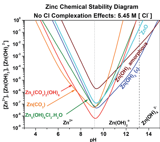
Fig. 3 Chemical stability diagram for the Zn–water system. Relevant species are given for exposure in a Cl - (5.45 M) and CO 3 2- (5.00 mM) containing environment. This diagram does not include the effect of ligand complexation due to the presence of Cl - .
