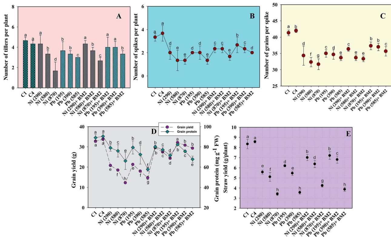
Fig. 6 Effect of three doses (mg kg -1 soil) of Ni and Pb (dose rates mentioned within brackets) on various parameters of wheat plants and bioremediation by metal tolerant B. subtilis BM2: number of tillers per plant (A); number of spikes per plant (B); number of grains per spike (C); grain yield and grain protein (D); straw yield (E). C1 and C4 represent uninoculated and Bacillus inoculated controls, respectively. Values denoted with different letters are significantly ( P \leq 0.05 ) different according to Duncan's multiple range test.
