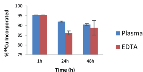
Fig. 2 Stability of AGuIX-NODAGA-IR783 ( 64 Cu) in plasma (blue) and upon EDTA challenge (red).
