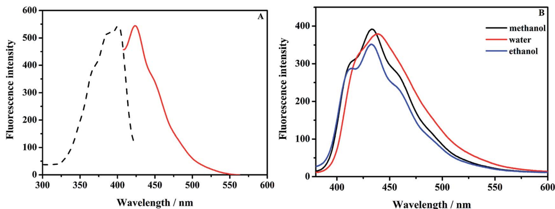
Fig. 1 (A) Fluorescence excitation (EX) and emission (EM) spectra of MNZ-F in methanol solution; (B) fluorescence emission spectra of MNZ-F in various solvents. ( \lambda_{\text{ex}} = 366 nm, sensitivity of 2, slit width of 10/10 nm).
