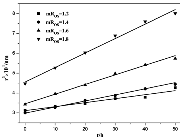
Fig. 11 The cube of the radius versus time for bifenthrin nanoemulsions at various mR_{OS} .
