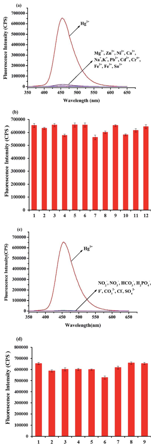
Fig. 5 (a) Fluorescence responses of probe HCDC (5 \mu\text{M} ) toward \text{Hg}^{2+} (5 \mu\text{M} ), and other metal ions (100 \mu\text{M} ). (b) Fluorescence responses of probe HCDC toward \text{Hg}^{2+} and in presence of other metal ions. (1) \text{Hg}^{2+} ; (2) \text{Mg}^{2+} ; (3) \text{Zn}^{2+} ; (4) \text{Sn}^{2+} ; (5) \text{Ca}^{2+} ; (6) \text{Na}^+ ; (7) \text{Fe}^{3+} ; (8) \text{Pb}^{2+} ; (9) \text{Cd}^{2+} ; (10) \text{Fe}^{2+} ; (11) \text{K}^+ ; (12) \text{Ni}^{2+} . (c) Fluorescence responses of probe HCDC (5 \mu\text{M} ) toward \text{Hg}^{2+} (5 \mu\text{M} ), and common anions species (100 \mu\text{M} ). (d) Fluorescence responses of probe HCDC toward \text{Hg}^{2+} and in presence of other common anions species (1) \text{Hg}^{2+} ; (2) \text{NO}_2^- ; (3) \text{NO}_3^- ; (4) \text{HCO}_3^- ; (5) \text{H}_2\text{PO}_4^- ; (6) \text{F}^- ; (7) \text{CO}_3^{2-} ; (8) \text{Cl}^- ; (9) \text{SO}_4^{2-} . The solution: in \text{H}_2\text{O}_2 (3 mM), HEPES (5 mM, pH 7.4) aqueous solution. Error bar = RSD ( n = 3 ).
