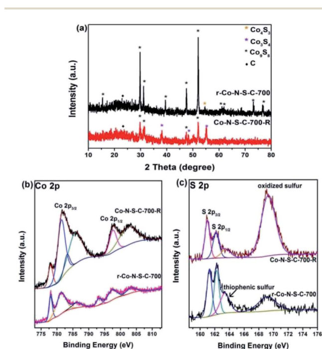
Fig. 4 (a) XRD patterns of r-Co-N-S-C-700 and Co-N-S-C-700-R; high-resolution XPS spectra of (b) Co 2p and (c) S 2p for Co-N-S-C-700-R (used) and r-Co-S-N-C-700 (re-activated).
