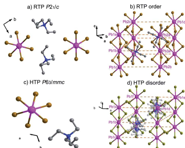
Fig. 2 (a) Molecular structures of complex 1 (296 K). (b) Packing diagram of complex 1 (296 K). (c) Molecular structures of complex 1 (393 K). (d) Packing diagram of complex 1 (393 K) (the hydrogen atoms bonded to the C atoms omitted for clarity).
