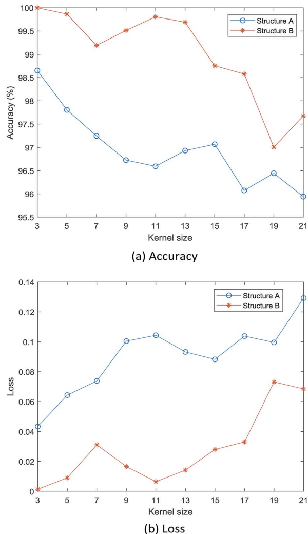
Fig. 4 Results of the 1D CNN model of the two structures under different convolution kernel sizes.
