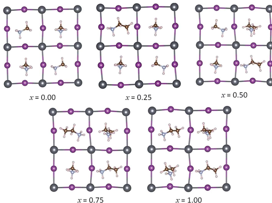
Fig. 2 Optimized stable geometries of the mixed MA_{1-x}EA_xPbI_3 perovskites.
