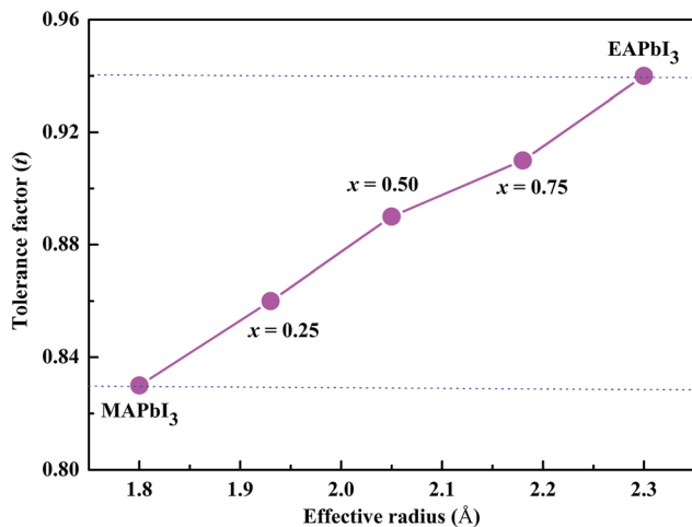
Fig. 1 Correlations between the tolerance factor and the structures of the MA_{1-x}EA_xPbI_3 perovskites.
