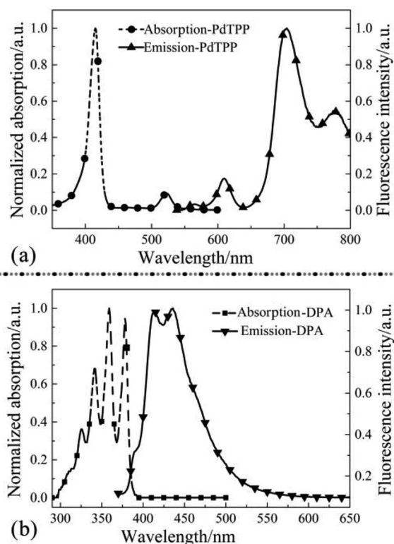
Fig. 1 Absorption and fluorescence spectra of PdTPP (a) and DPA (b) with solvent toluene at a concentration of 1 \times 10^{-6} \text{ mol L}^{-1} .
