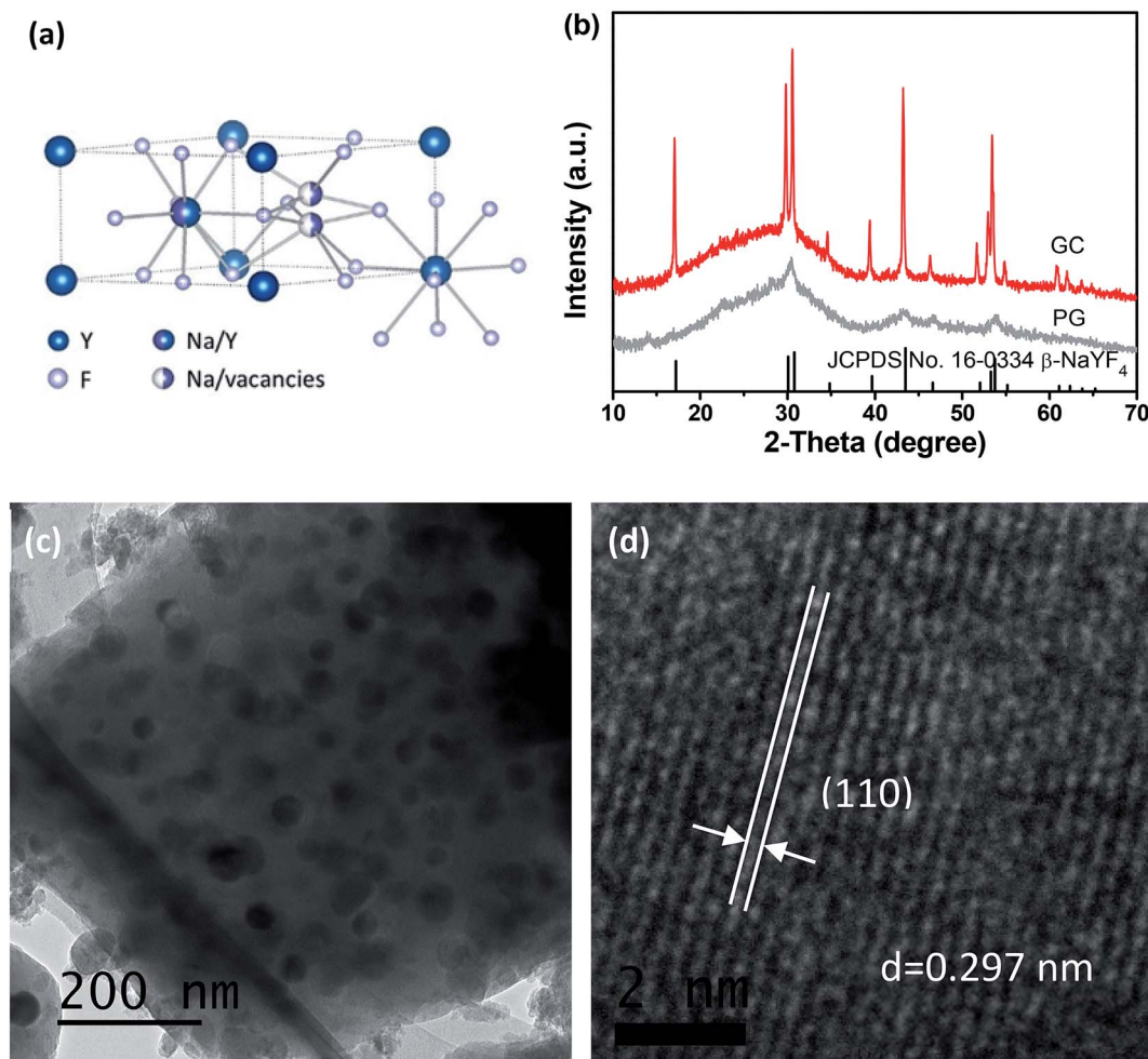
Fig. 1 (a) Crystal structure of \beta - \text{NaYF}_4 . (b) XRD patterns of PG and GC samples with standard card of \beta - \text{NaYF}_4 (JCPDS no. 16–0334). (c) TEM and (d) HRTEM of \beta - \text{NaYF}_4 nanocrystal embedded glass ceramics.
