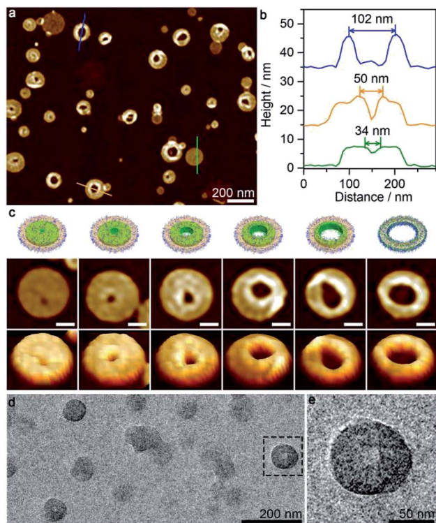
Fig. 5 (a) AFM height images and (b) height profiles of perforated disk-like micelles formed by the self-assembly of PS 580 - b -PB 660 - b -P2VP 920 at acetone/cyclohexane = 65/35. (c) Schematic representations, AFM height images and 3D images showing the perforated disk-like micelles with various hole sizes. The scale bars correspond to 50 nm. (d and e) TEM images of perforated disk-like micelles.
