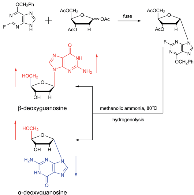
Fig. 8 First synthesis of α-deoxyguanosine.
