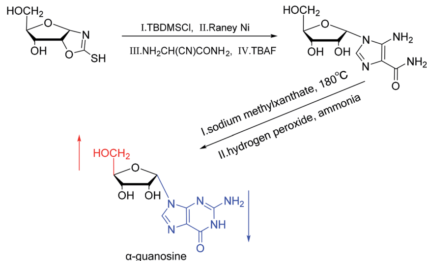
Fig. 7 First synthesis of α-guanosine.
