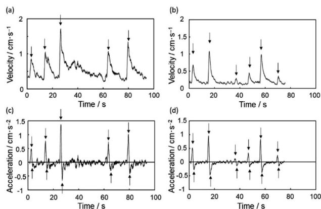
Fig. 6 The motion of upward pin is shown with (a) velocity and (c) acceleration. The NIR is irradiated 5 times around arrows. The motion of downward pin is shown with (b) velocity and (d) acceleration. The NIR is irradiated 6 times around arrows.
