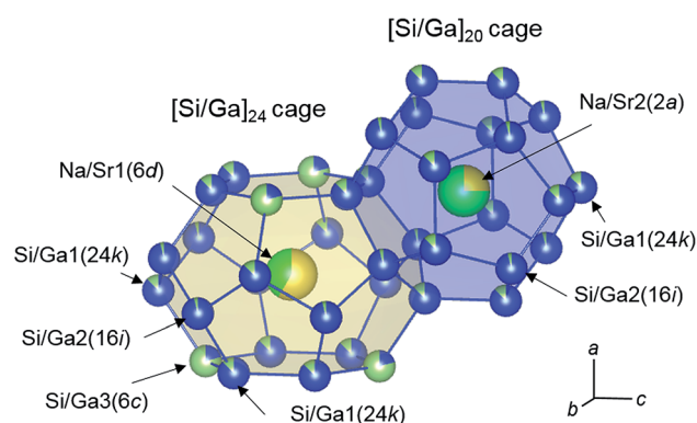
Fig. 3 Structures of the [Si/Ga] 20 and [Si/Ga] 24 cages of \text{Na}_{3.9}\text{Sr}_{4.1}\text{Ga}_{9.1}\text{Si}_{36.9} (Na: yellow, Ga: yellow-green, Si: blue, Sr: green). The occupancies are represented by the surface areas of the spheres.
