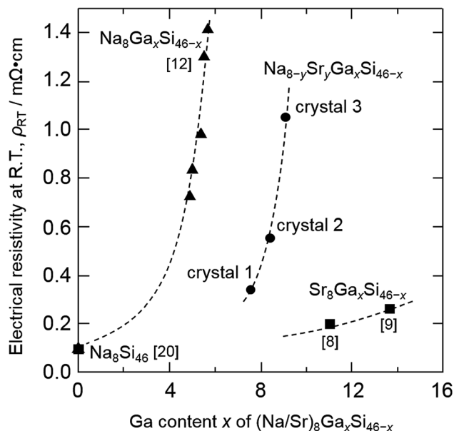
Fig. 5 Electrical resistivity at room temperature versus Ga content of type-I clathrates: Na 8 Si 46 , 20 Na 8 Ga x Si 46-x , 12 Sr 8 Ga x Si 46-x , 8,9 and Na 8-y Sr y Ga x Si 46-x crystals 1 (Na 5.0 Sr 3.0 Ga 7.6 Si 38.4 ) and 2 (Na 4.2 Sr 3.8 Ga 8.4 Si 37.6 ), and 3 (Na 3.9 Sr 4.1 Ga 9.1 Si 36.9 ).
