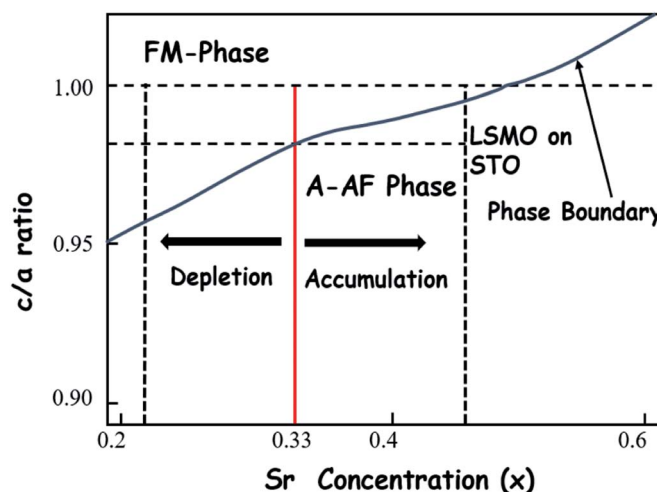
Fig. 4 Phase diagram of LSMO as a function of Sr concentration ( x ) and tetragonal ratio c/a . 69 LSMO experiences a compressive strain when grown on STO. The phase transitions due to accumulation and depletion of holes in LSMO and varied tetragonal ratios of the sample are shown. 69,71
