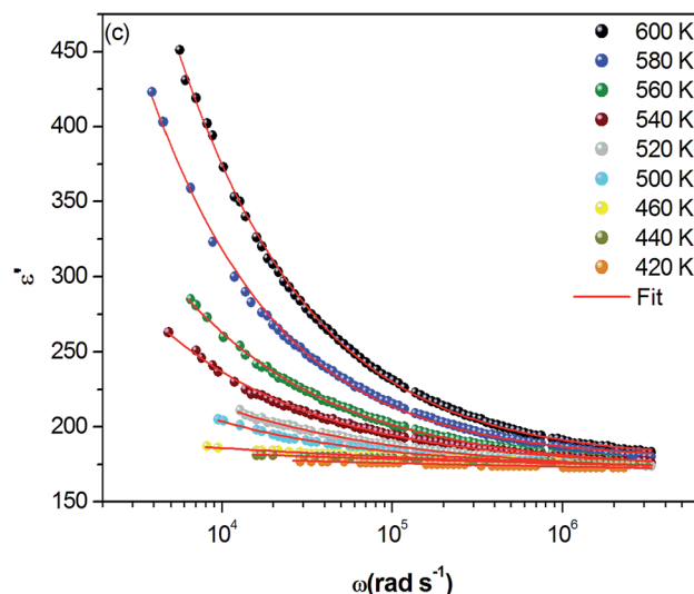
Fig. 8 (a, b and c) Frequency dependence of the real part of the dielectric constant, \varepsilon' at different temperatures for \alpha -NaCoPO 4 , \beta -NaCoPO 4 and \gamma -NaCoPO 4 respectively.
