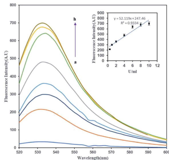
Fig. 2 The fluorescence spectra of ( 1 \text{ mg mL}^{-1} ) of FAM-oligo-Au dsDNA probe methylation upon treated with a series of concentration of M.SssI MTase enzyme (a-h: 0, 0.5, 1, 2, 4, 6, 8, 10 \text{U mL}^{-1} ). Inset shows standard curve of relative fluorescence intensity versus M.SssI MTase enzyme concentration.
