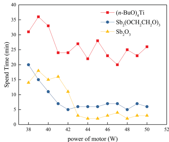
Fig. 1 Reaction spend time of different catalysts for per watt. (The molar amounts of the metals are the same in polymerization of different catalysts.)
