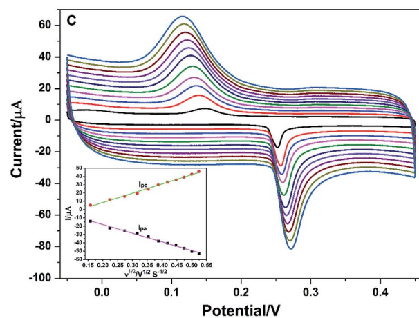
Fig. 4 (A) Cyclic voltammograms of 4.0 \mu\text{M Cu}^{2+} in 0.1 \text{ M PBS} (pH 6.5) at different scan rates on PG/GCE. (B) Cyclic voltammograms of 4.0 \mu\text{M Cd}^{2+} in 0.1 \text{ M PBS} (pH 6.5) at different scan rates on PG/GCE. (C) Cyclic voltammograms of 2.0 \mu\text{M Hg}^{2+} in 0.1 \text{ M PBS} (pH 6.5) at different scan rates on PG/GCE. Inset: plot of peak currents ( I_{pa} and I_{pc} ) against the scan rate ( \nu ).
