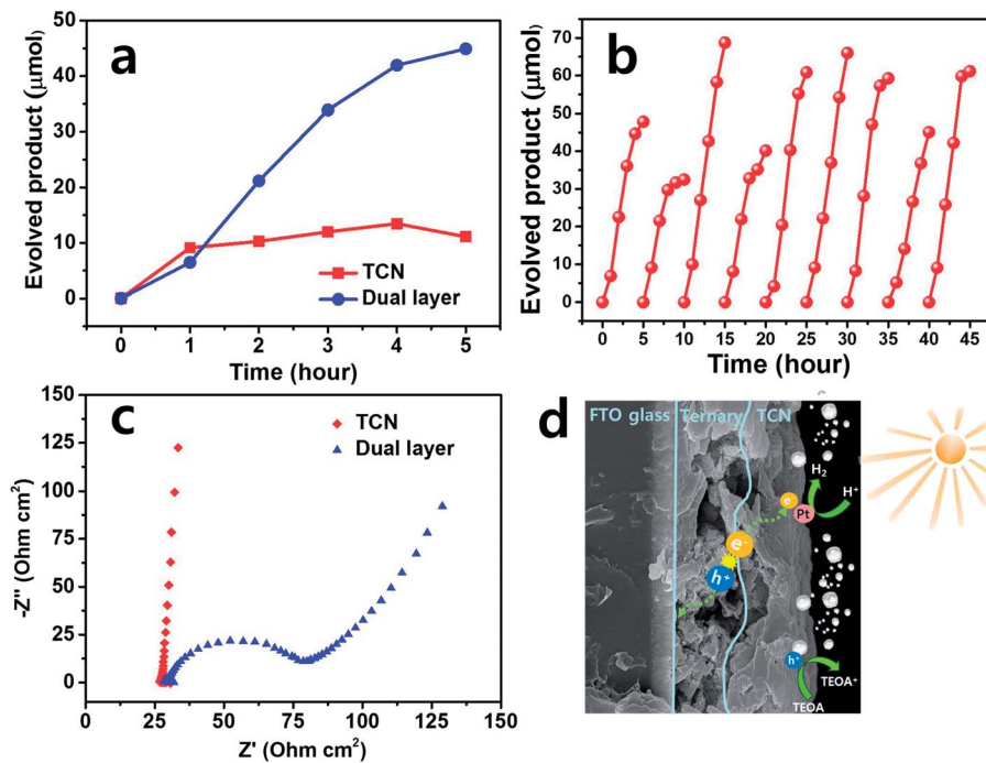
Fig. 5 (a) Hydrogen (H 2 ) evolution on TCN film and dual layered film, (b) H 2 evolution recycle tests on dual layered film, (c) electrochemical impedance spectroscopy (EIS) measurement on TCN film and dual layered film and (d) its possible mechanism.
