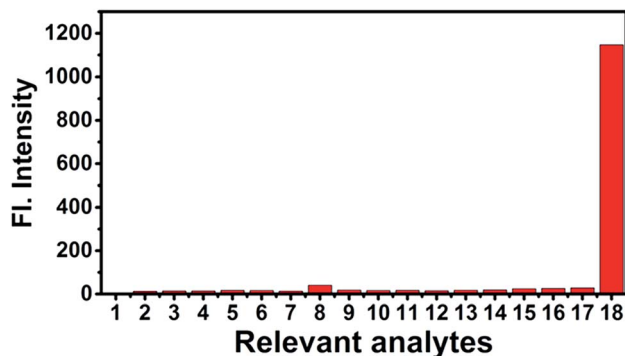
Fig. 4 Fluorescence spectra of NS-C1O (10 \mu M) in pH 7.4 PBS buffer (containing 5% DMF) for various relevant species (50 \mu M). 1: None; 2: GSH; 3: Cys; 4: Hcy; 5: F - ; 6: Cl - ; 7: Br - ; 8: \cdot OH; 9: ONOO - ; 10: DTBP; 11: TBHP; 12: NO; 13: H 2 O 2 ; 14: NO 2 - ; 15: Co 2+ ; 16: Cu 2+ ; 17: Ni 2+ ; 18: ClO - .
